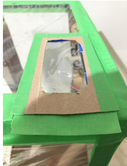
10. Tape the pocket to a corner on the roof. Use two sides of the frame to provide support for the ventilation gate holder.
